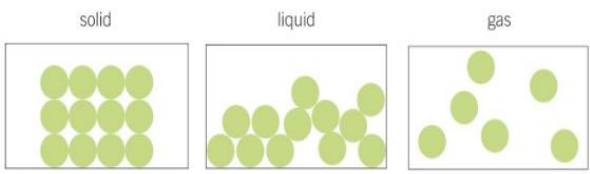
▲ The arrangement of particles explains the speed of sound in different materials.
