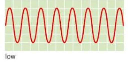
▲ A high sound has a higher frequency than a low sound.
