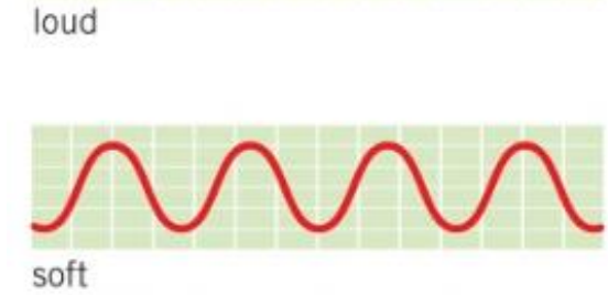
▲ A loud sound has a bigger amplitude than a soft sound.
